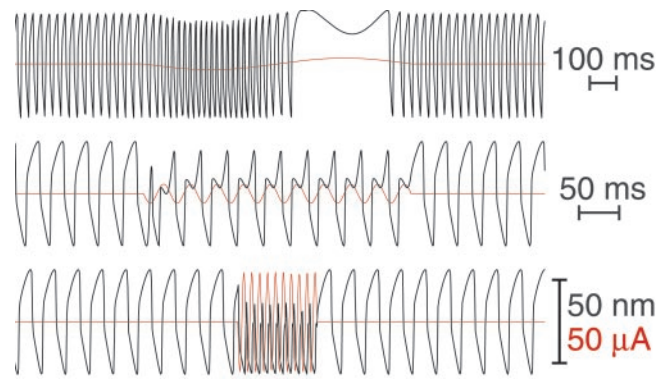
Fig. 4. Modeling of electrically evoked hair-bundle movements. Stimulation at 1 Hz ( Top ) accelerated bundle oscillation during the negative phase of stimulation and arrested movement during the positive phase. Excitation with a 30-Hz current ( Middle ) mimicked the intermediate regime of bundle responsiveness, with complex but phase-locked bundle movements. The modeled response to 100-Hz stimulation ( Bottom ) displays phase-locking, with movements of a polarity opposite that of stimulation. The three records correspond to those for the same stimulus frequencies in Fig. 1A. Except for the frequency and amplitude of stimulation, the values of all parameters in the model were identical in the three simulations. The uppermost time calibration refers to the top record and the second calibration to both subsequent records; the distance and current calibrations apply to all three records.
