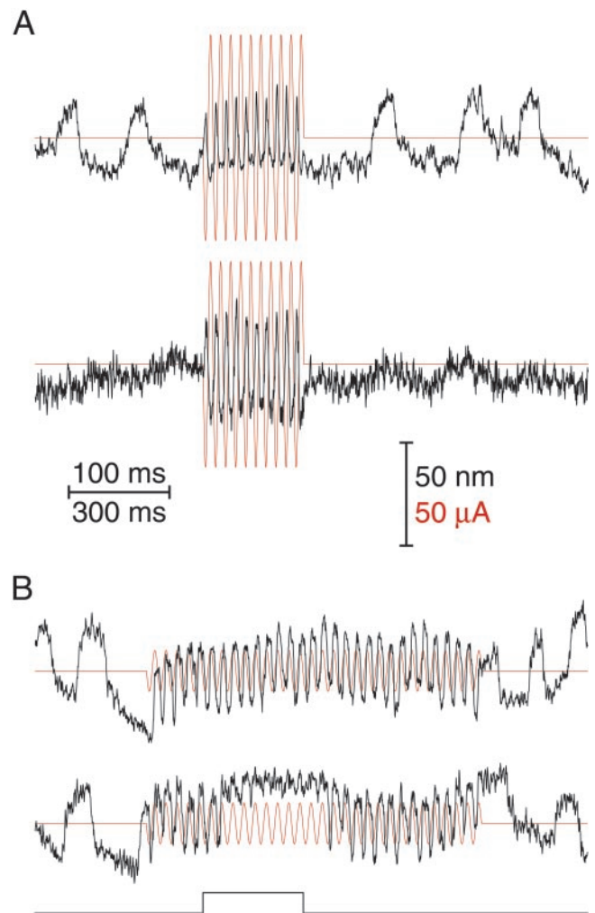
Fig. 3. Effects of butanedione monoxime and gentamicin on electrically evoked hair-bundle movements. (A) Under control conditions, a hair bundle oscillated spontaneously and responded to electrical stimulation at 100 Hz (Upper). In the presence of 20 mM butanedione monoxime, the same bundle produced a comparable electrical response without spontaneous oscillation (Lower). The high-frequency spikes of bundle motion in the latter record might reflect the residual activity of myosin molecules. (B) A spontaneously active hair bundle responded well under control conditions to 30-Hz electrical stimulation (Upper). The electrical response was blocked when the same bundle was exposed to gentamicin (Lower), whose iontophoretic application is indicated beneath the recording. Drug exposure offset the bundle in the positive direction, an indication of blockage in the open-channel state.
