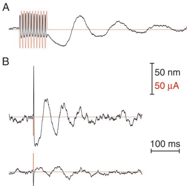
Fig. 2. Time scales of hair-bundle responsiveness to electrical stimulation. (A) Application of 10 cycles of 100-Hz electrical current entrained the motion of the bundle, eliciting movements of a polarity opposite that of the stimulus. After cessation of the stimulus, a damped oscillation occurred at the cell's natural frequency of \approx 7 Hz. (B) Electrical pulses 1 ms in duration elicited rapid mechanical responses of opposite polarity, followed by a slower oscillation at the natural frequency of the cell of \approx 16 Hz. Note the asymmetry in the responses to negative (Upper) and positive (Lower) stimuli. Each of the three records displays the average of 50 successive measurements.
