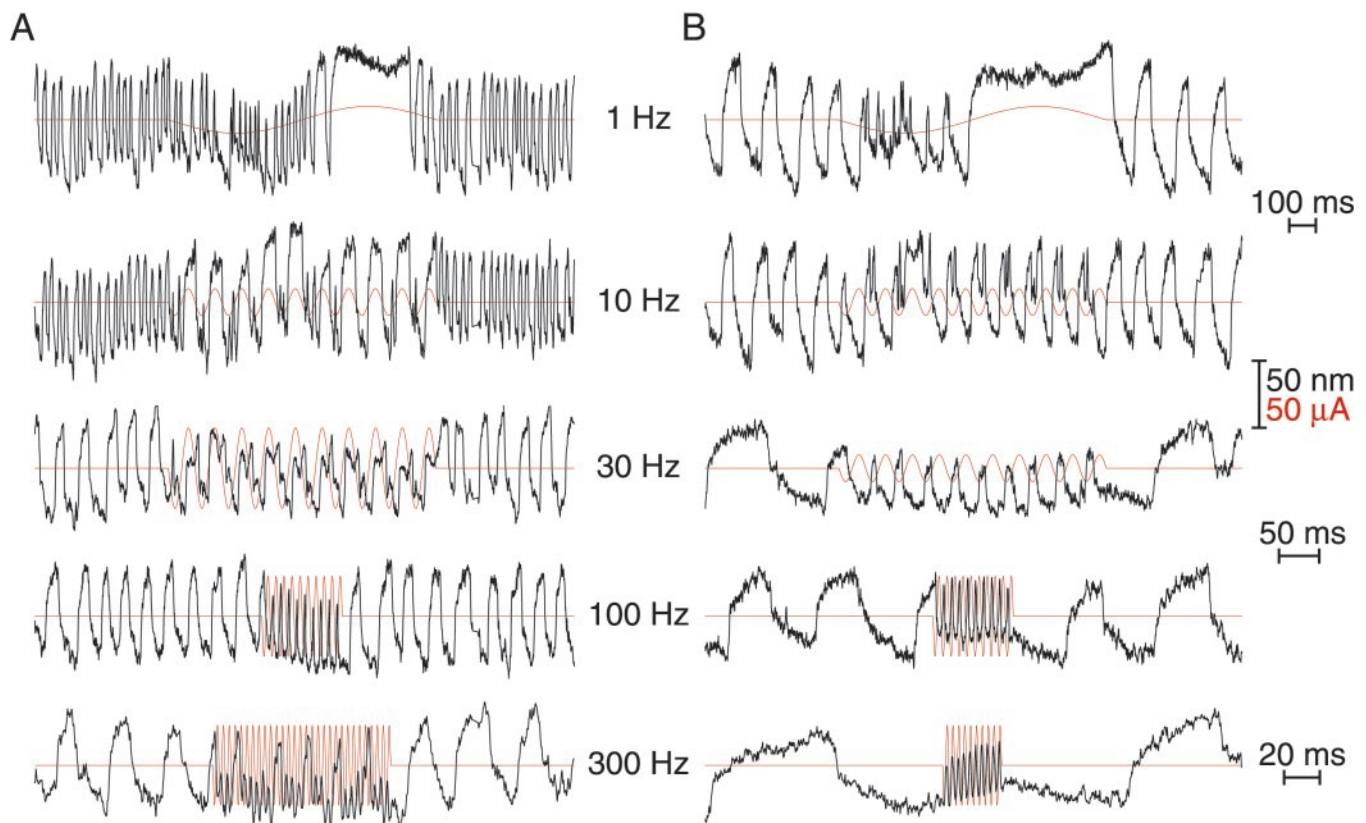
Fig. 1. Response of active hair bundles to stimulation by sinusoidal transepithelial current. (A) Before stimulation, a hair bundle oscillated spontaneously at \approx 35 Hz. During negative stimulation at 1 Hz, the bundle displayed faster and smaller oscillations with occasional omissions; the positive stimulus phase slowed and eventually blocked oscillatory movements. Similar responses occurred during stimulation at 10 Hz. At 30 Hz, slightly below the natural frequency of the cell, the response comprised phase-locked movements adorned with complex spikes. At 100 and 300 Hz, the response was essentially out of phase with the stimulus. During a 300-Hz stimulation, spontaneous bundle oscillations resumed, superimposed on the rapid, phase-locked response. (B) The hair bundle of a second cell oscillated spontaneously at \approx 8 Hz. Although electrical stimulation evoked responses similar to those in A, the transition from the low- to the intermediate-frequency regime of responsiveness occurred at a frequency < 10 Hz. In this and the subsequent figures, each mechanical response is superimposed on a record of the electrical stimulus (red). Positive bundle movement is defined as that towards the kinocilium. Positive current is defined as that depolarizing the apical membrane of the hair cell. The top time calibration applies to the 1- and 10-Hz records, the middle calibration corresponds to the 30- and 100-Hz records, and the bottom calibration refers only to the 300-Hz records.
