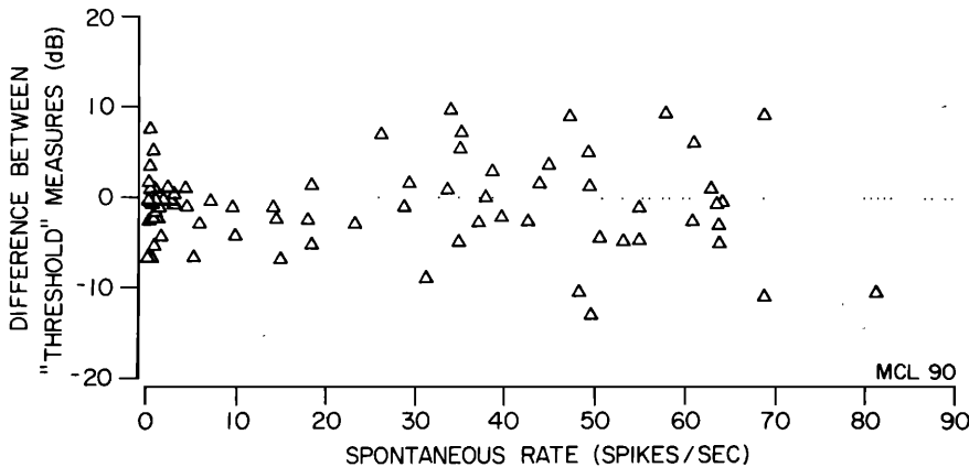
FIG. 1. Effect of spontaneous rate on the performance of the tuning-curve algorithm. The data are from one routine-normal animal in which the tuning curves were determined with a "criterion" of 0. Each point represents data from a different unit. The abscissa represents the difference between the "threshold" at CF as determined by the algorithm and the intensity required (as determined from the rate-level function) to increase the unit's firing rate by 10 spikes/s. A positive value of the abscissa indicates that the algorithm registered a threshold level which was higher than that required to produce the predicted rate increase. In this and all subsequent figures, the spontaneous rate represents the average rate as determined over a 30-s sample.
