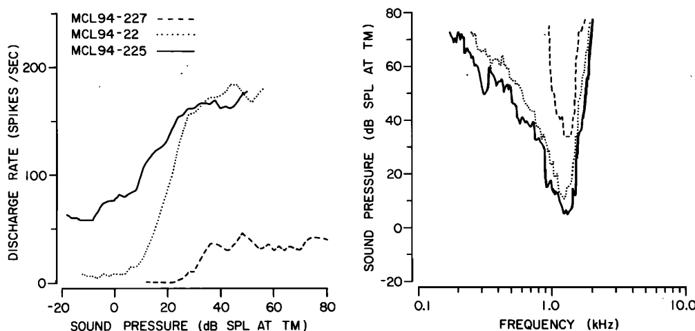
FIG. 16. Typical rate-level functions at the CF for units from the three spont classes in one of the chamber-raised animals. The tuning curves for the three units (criterion 0) are shown in the right-hand panel. The rate-level functions (left) have undergone three-point smoothing. The spont rate for units 227, 22, and 225 were 0.03, 3.83, and 56.3 spikes/s, respectively.
