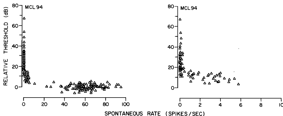
FIG. 10. Relation between spont and relative threshold in one of the chamber-raised animals. In the right panel the data from the low-rate units are displayed on an expanded horizontal scale. The relative threshold of each unit is the difference between its threshold at CF and the average threshold at CF of all the units from the same ear with similar CF and with rates of spontaneous discharge greater than 18 spikes/s. The normalization curve describing the average threshold as a function of CF was derived by dividing the CF continuum into 40 logarithmically spaced frequency bins, averaging the thresholds at CF for all the "high-spont" units within each CF bin and interpolating between the 40 mean-threshold values thus derived. Excluded from these scatter plots are those units with CF below 0.4 or above 15 kHz. Absolute threshold measurements were made with the automated tuning-curve program at criterion 0.
