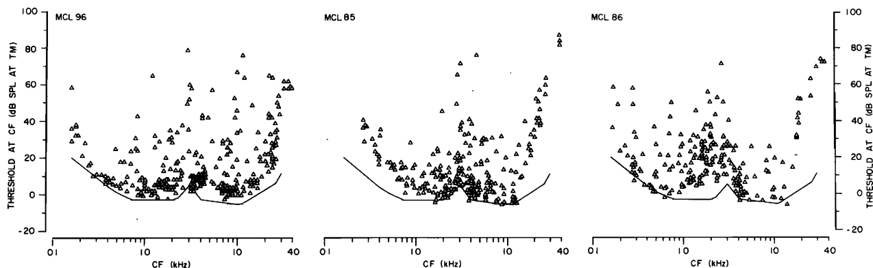
FIG. 2. Distribution of thresholds at CF obtained in three different cats. Each panel plots the threshold at the CF for each of the units encountered in one animal. For each unit, the "threshold" is that value obtained by the automated tuning-curve paradigm with a criterion of 1. The case in the left panel (MCL96) was one of the animals raised in the soundproofed room. The other two cases were cats from the population routinely available to us as experimental animals. Superimposed on the data from each animal is the "best-threshold curve," or BTC (see text). Since the BTC has been smoothed, some of the data points in MCL85 and 86 fall a few decibels below the curve. In this and all subsequent figures the sound pressure levels are expressed in decibels re 0.0002 dyn/cm 2 , as measured near the tympanic membrane (TM).
