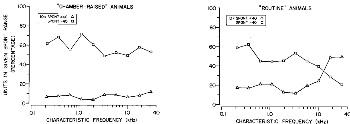
FIG. 7. Compression of the spont rate distribution at high CF in routine animals. The data in the left panel are from three chamber-raised cats (MCL93, MCL94, and MCL96). The data on the right are from 14 animals among those routinely available from local suppliers (MCL14, 47, 49, 75, 79–86, 89, and 90). To make each curve, the units in the sample were divided according to CF into ten logarithmically spaced frequency bins. Each box represents the percentage of units in that CF bin which had spont greater than 40 spikes/s; each triangle represents the percentage of units with spont between 10 and 40 spikes/s. Each symbol is placed in the center of the appropriate CF bin.
