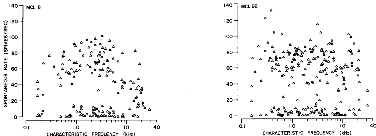
FIG. 4. Distribution of spontaneous rates as a function of CF in each of two routine-normal animals. Each point represents data from a different single unit. Each panel displays all the data obtained from each animal.
