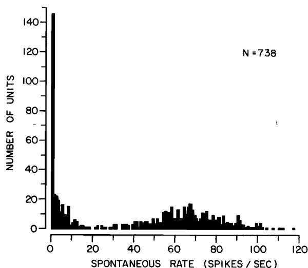
FIG. 9. Histogram of spontaneous rates sampled from the three most sensitive chamber-raised cats (MCL93, 94, 96). The bin width for the histogram is 1 spike/s. The "N" refers to the number of units in the sample.
