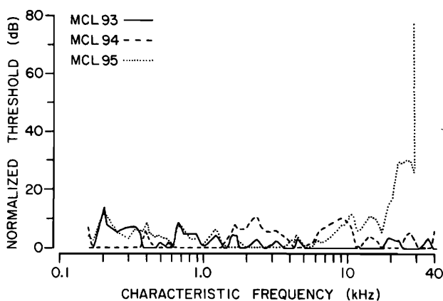
FIG. 8. Comparison of minimum-threshold envelopes for the unit samples in each of three chamber-raised cats. To make these comparisons the curve representing, as a function of CF, the minimum threshold at CF was drawn for each of the three chamber-raised cats for which the automated tuning curves were run at criterion 0. Since the unit sample in each of these animals included better than 250 units, and since these samples were well distributed across CF, there was little ambiguity as to how such minimum-threshold curves should be drawn. The curve for each animal, as it appears in the figure, has been normalized with respect to the minimum-threshold envelope for the entire sample from these three experiments.
