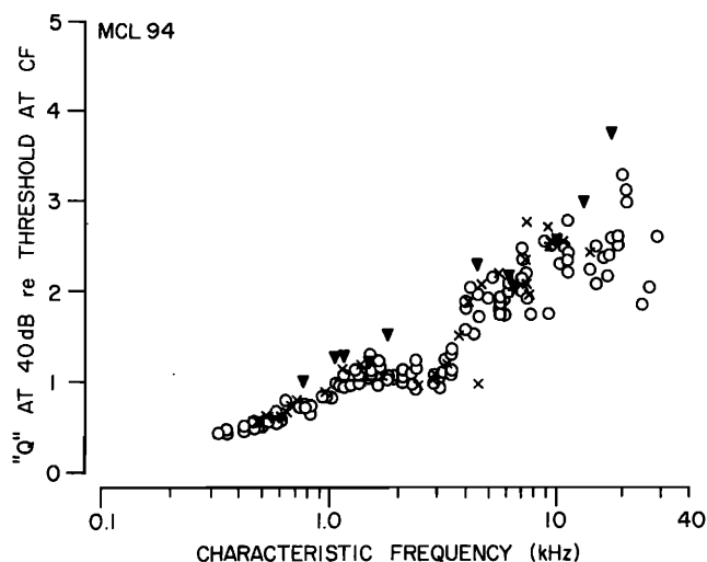
FIG. 14. Tuning curve "Q" as a function of CF with coding for spont rate. "Q" is measured at 40 dB re threshold at CF and is defined as the ratio of the characteristic frequency to the bandwidth of the tuning curve. Solid triangles represent low-spont units, crosses represent medium-spont units, and open circles represent high-spont units. The data are taken from one of the chamber-raised animals.
